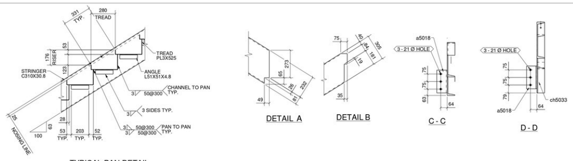
TYPICAL PAN DETAIL
